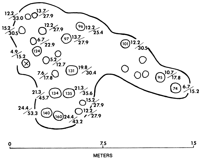
FIGURE 5. Spatial distribution, height, and diameters of trees in one of the older copes at Paradise Valley, Mount Rainier National Park, Wash. Numbers within circles are ages; numbers outside of circles are total heights and diameters at breast height, e.g., 24.0/43.0 = 24 m tall and 43 cm d.b.h. Trees marked with "X" are dead.
